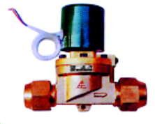
FDF- 制冷电磁阀 refrigeration solenoid valve
