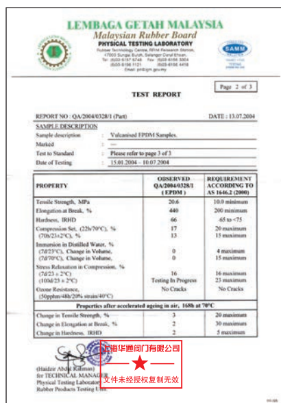
★ 橡胶试片硫化测试 Testing of Vulcanization Rubber Test Pieces
